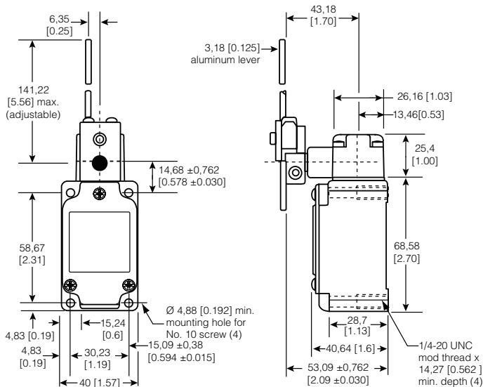
Figure 3. 1LS10 Dimensions
