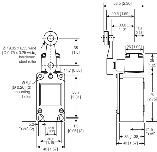
Figure 25. 1LS3-4 Dimensions
