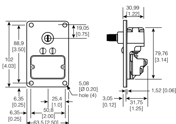
Figure 7. 7LS1 Dimensions
