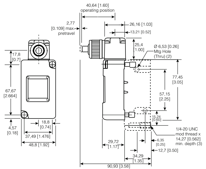
Figure 18. 205LS1 Dimensions
