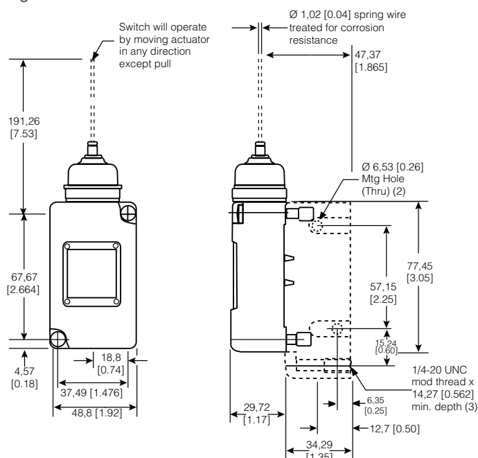
Figure 22. 208LS125 Dimensions
