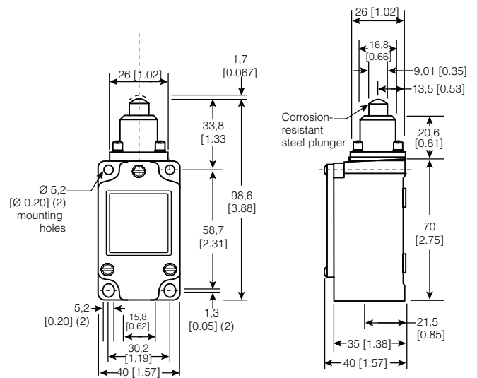
Figure 28. 4LS1-4 Dimensions
