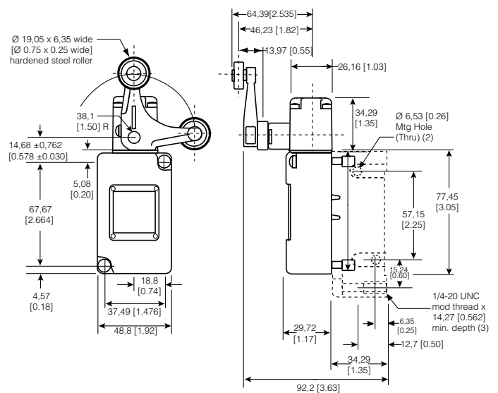
Figure 19. 206LS1 Dimensions
