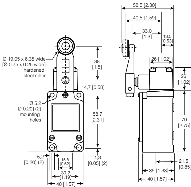
Figure 25. 1LS3-4 Dimensions
