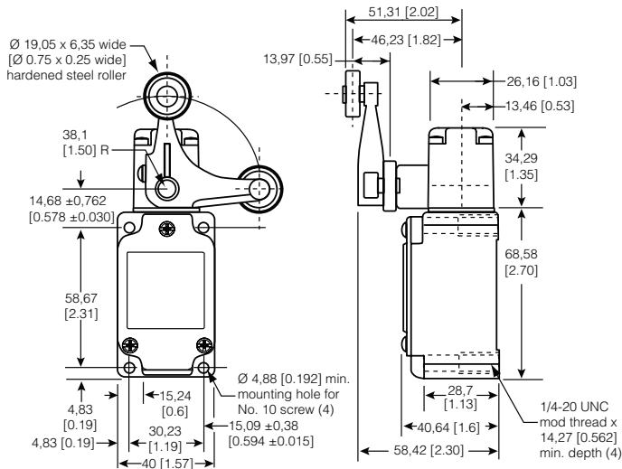
Figure 6. 6LS1 Dimensions
