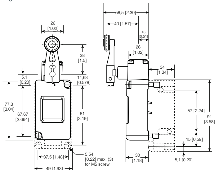
Figure 36. 202LS1-4 Dimensions
