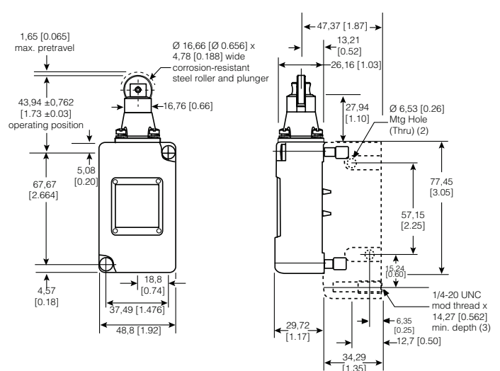
Figure 19. 206LS1 Dimensions
