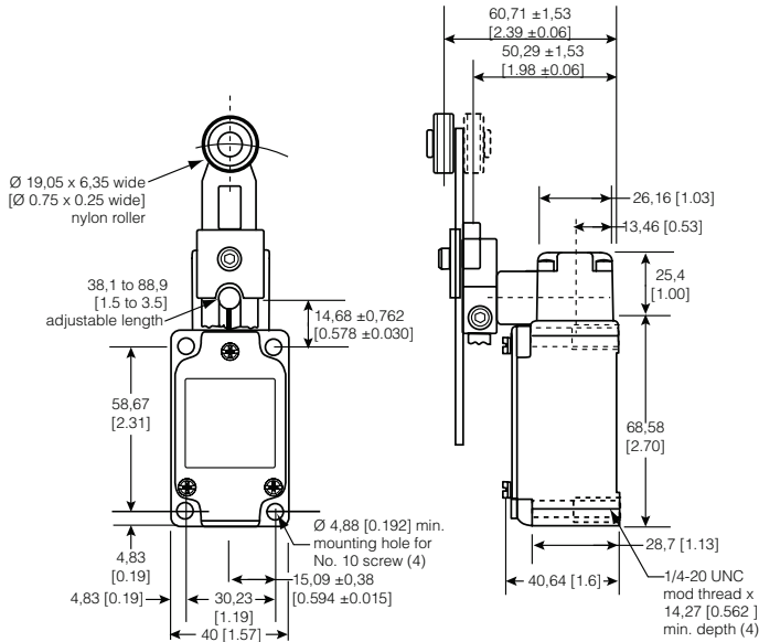
Figure 3. 1LS10 Dimensions
