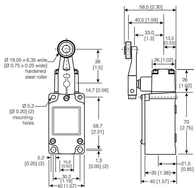
Figure 27. 2LS1-4 Dimensions
