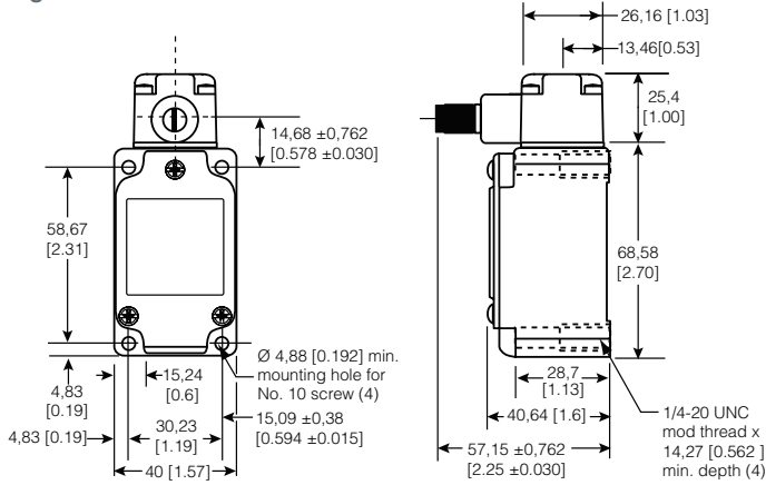
Figure 2. 1LS3 Dimensions
