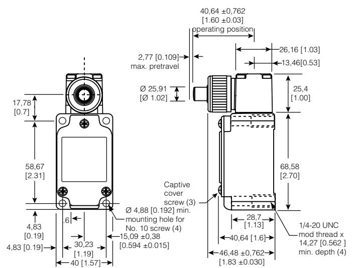
Figure 6. 4LS1 Dimensions
