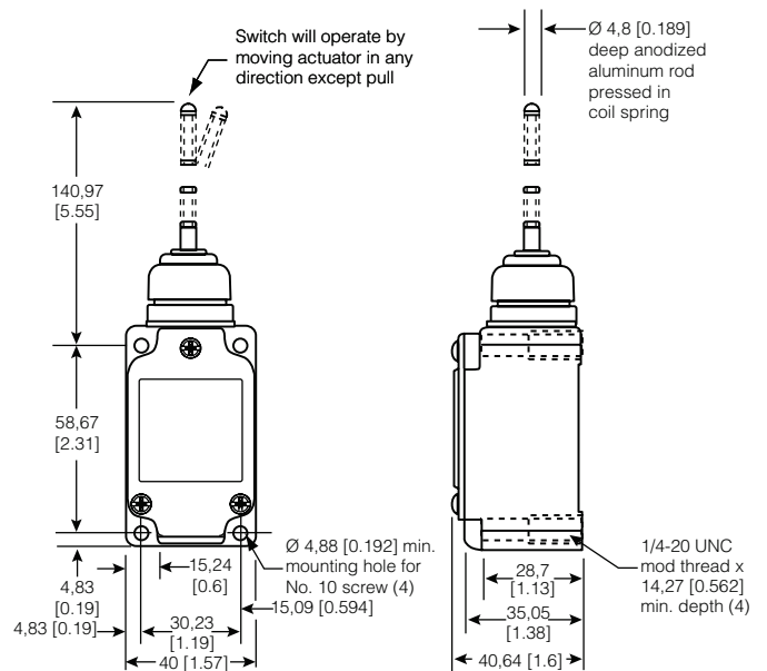
Figure 9. 8LS3 Dimensions
