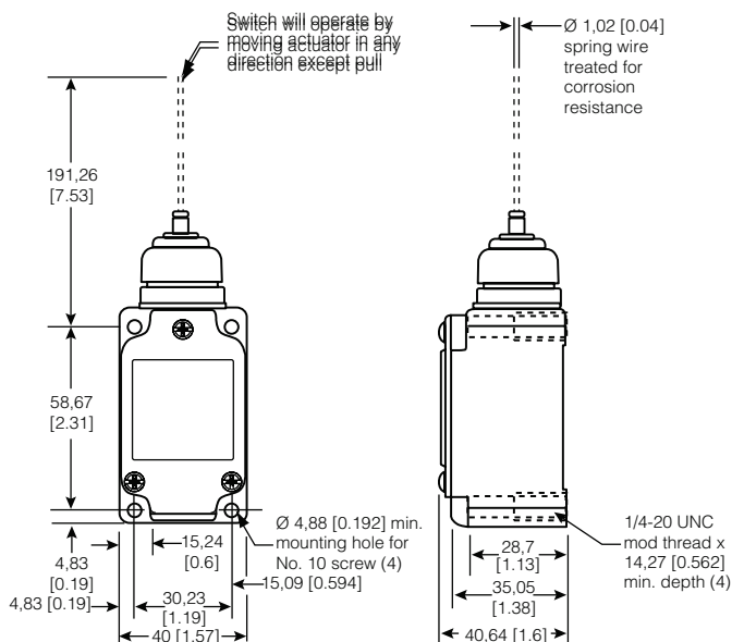
Figure 11. 8LS152 Dimensions
