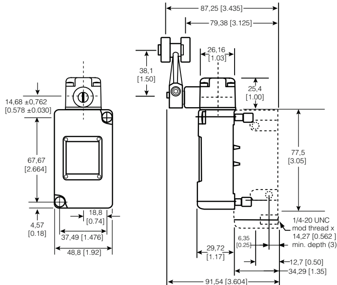
Figure 13. 201LS3 Dimensions
