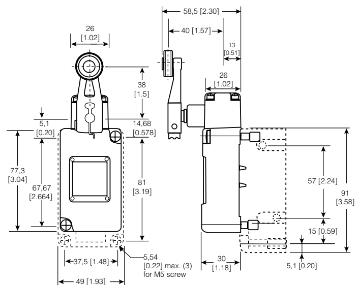
Figure 34. 201LS3-4 Dimensions
