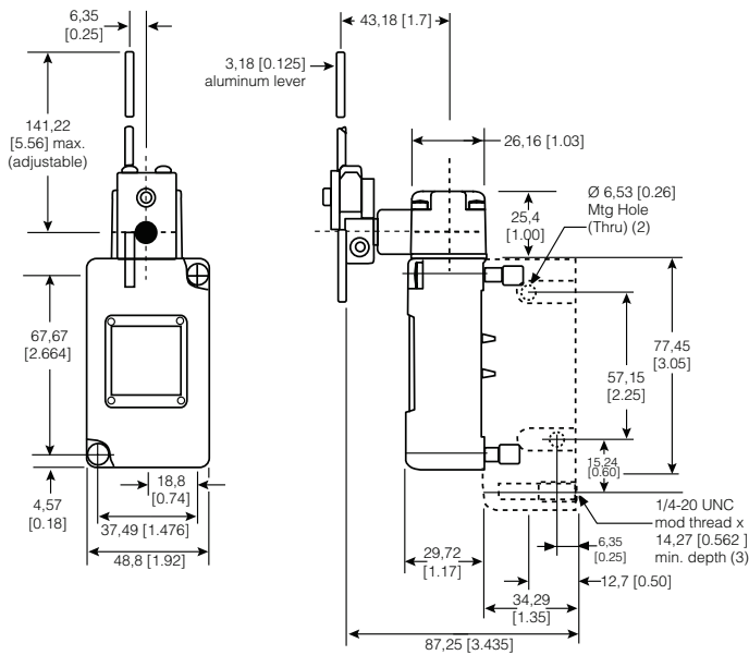
Figure 15. 202LS1 Dimensions
