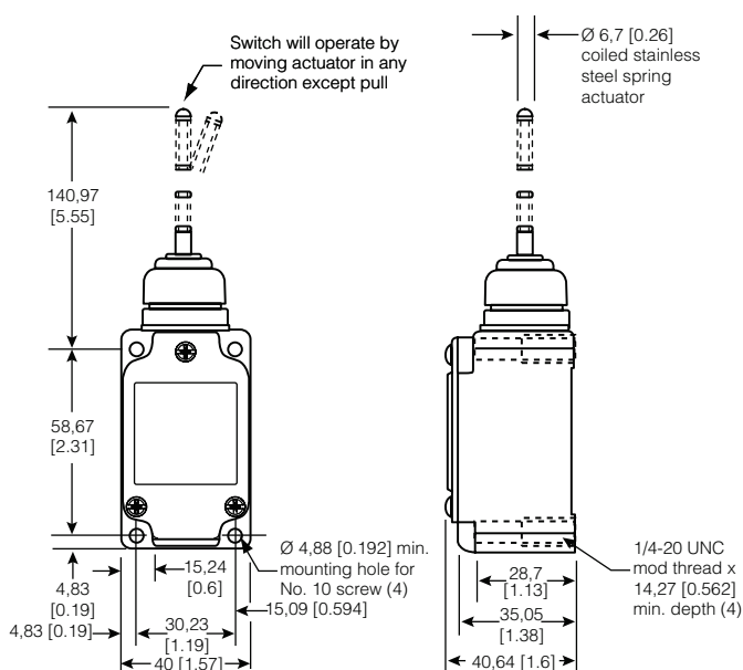
Figure 11. 8LS152 Dimensions
