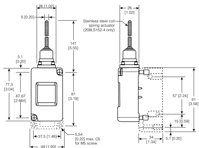
Figure 39. 208LS1-4 Dimensions
