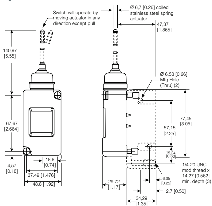
Figure 23. 208LS152 Dimensions
