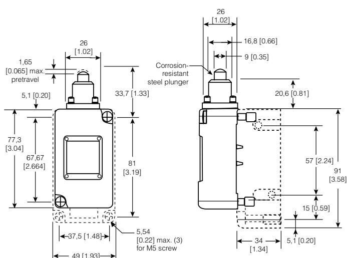
Figure 37. 204LS1-4 Dimensions
