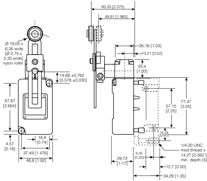
Figure 13. 201LS3 Dimensions
