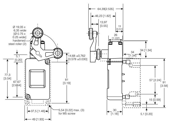
Figure 34. 201LS3-4 Dimensions
