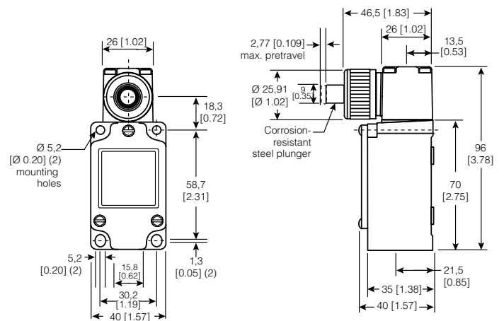
Figure 28. 4LS1-4 Dimensions
