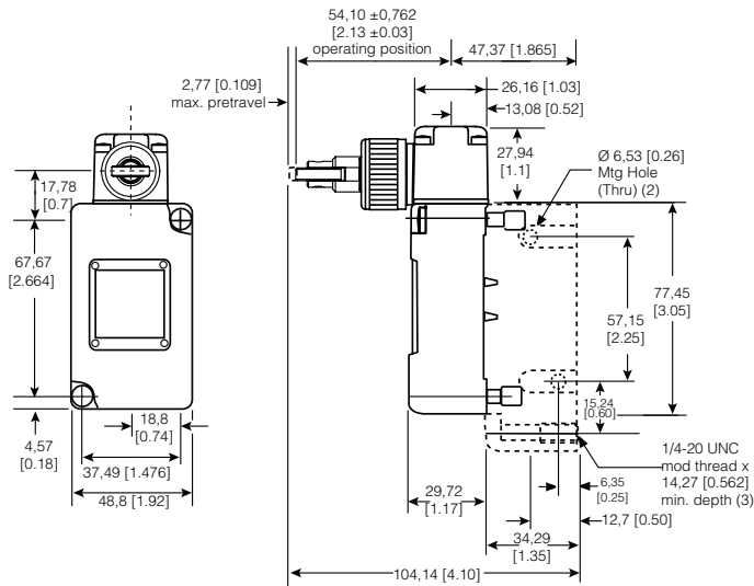
Figure 16. 203LS1 Dimensions
