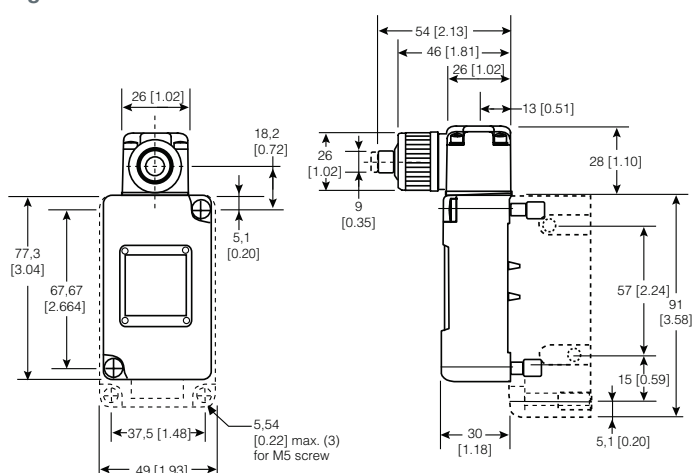
Figure 37. 204LS1-4 Dimensions
