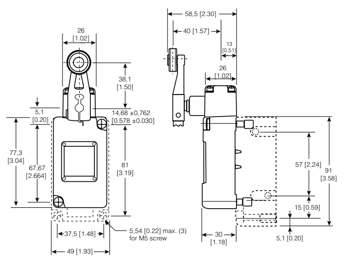
Figure 33. 206LS1-4 Dimensions
