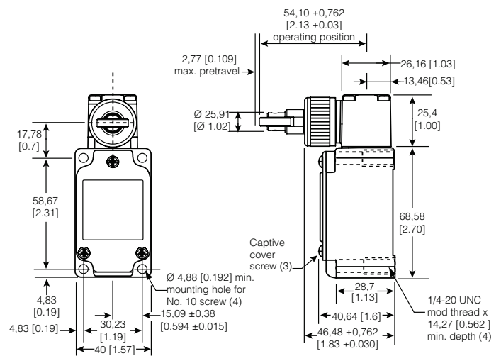
Figure 6. 4LS1 Dimensions
