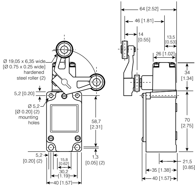
Figure 31. 8LS1-4 Dimensions
