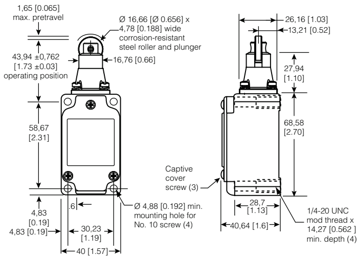
Figure 7. 5LS1 Dimensions
