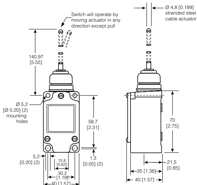
Figure 31. 8LS1-4 Dimensions
