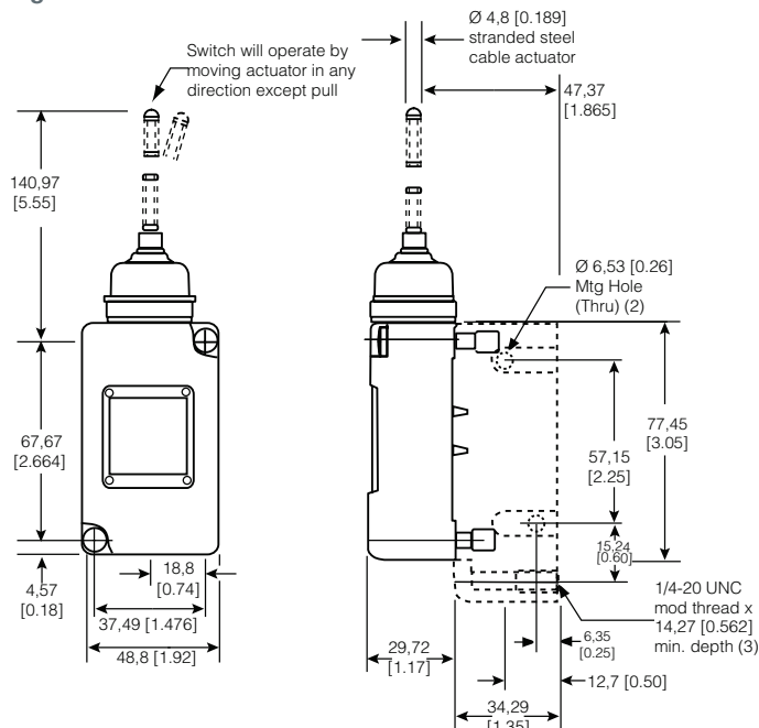
Figure 20. 208LS1 Dimensions
