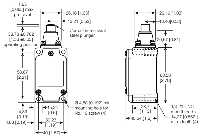
Figure 5. 3LS1 Dimensions
