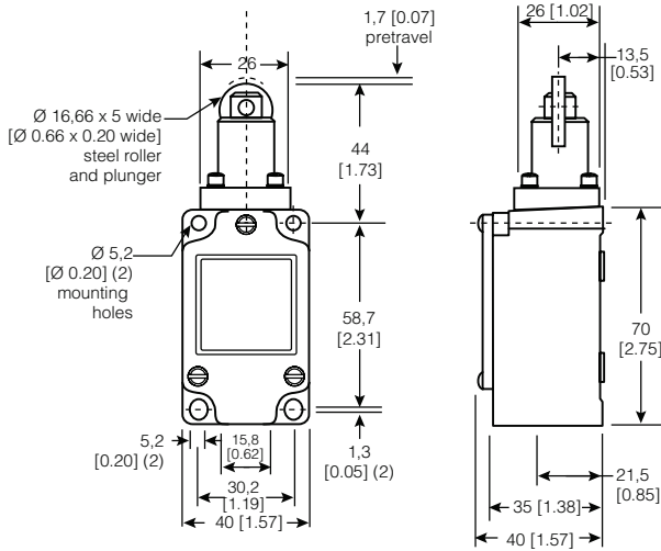
Figure 30. 6LS1-4 Dimensions
