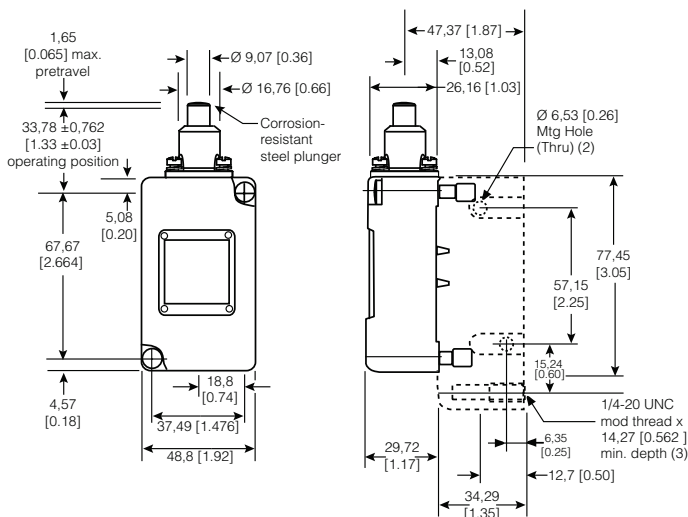
Figure 16. 203LS1 Dimensions
