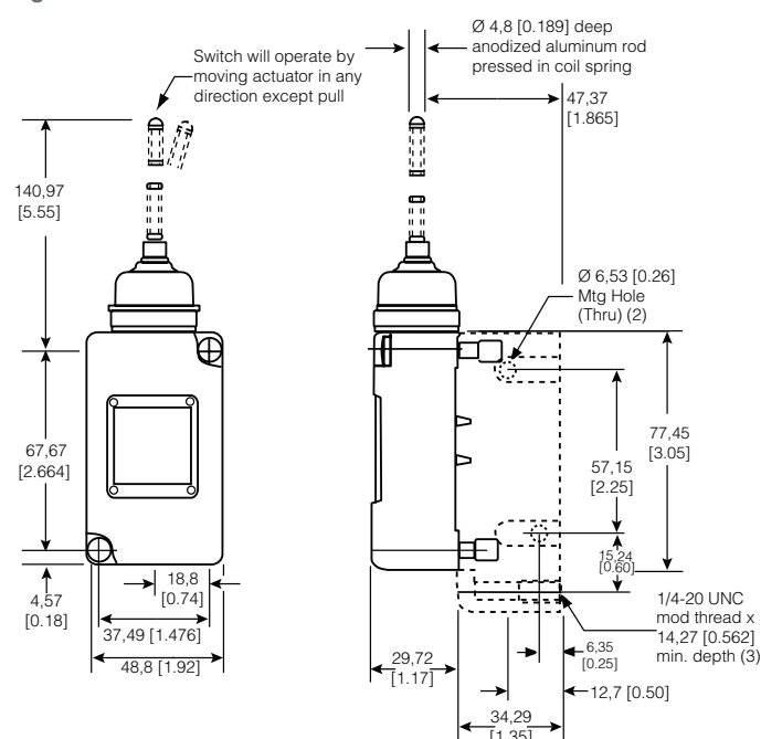
Figure 21. 208LS3 Dimensions
