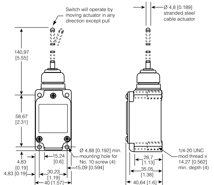
Figure 8. 8LS1 Dimensions
