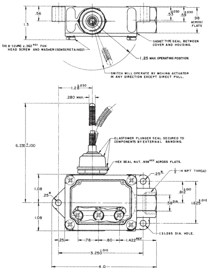
Figure 6. Flexible rod: BAF1/DTF1-2RN18-XX (left-hand version shown)
