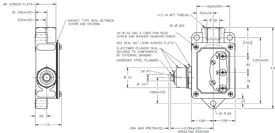
Figure 2. Roller Plunger: BAF1/DTF-2RQ9-XX (left-hand version shown)
