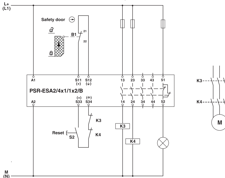
Circuit diagram
